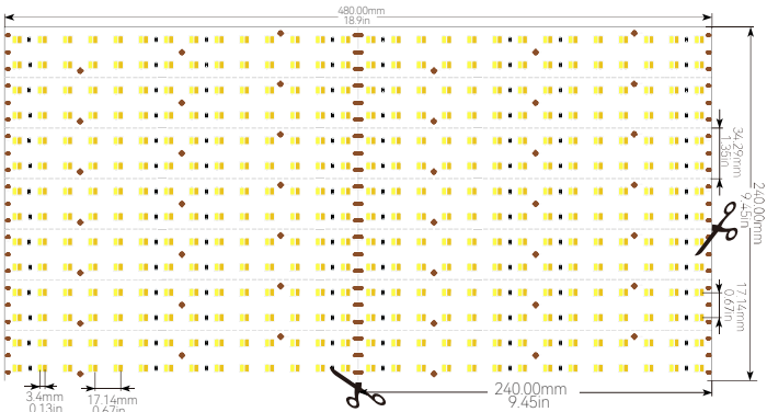
Dimension Cuttable Flex Mat, 784LEDs, DC48V
