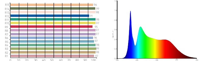
CINEMA DAYLIGHT COLOR RENDERING INDEX 6560K Ra=97.7
