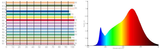
CINEMA TUNGSTEN COLOR RENDERING INDEX 2787K Ra=97.7
